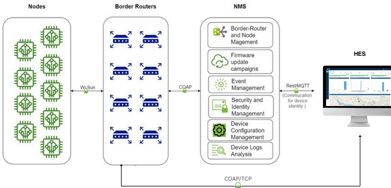
NMS End-to-End Architecture (For Transportation Layer Communication )
